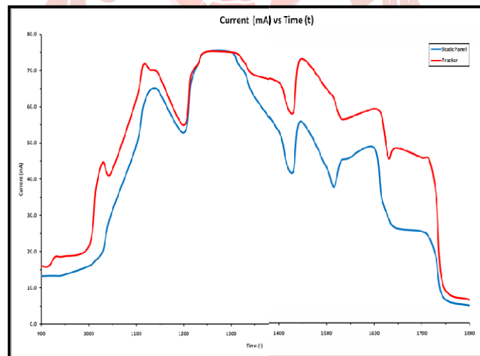
Figure 9. Output power comparison between static panel and tracker
