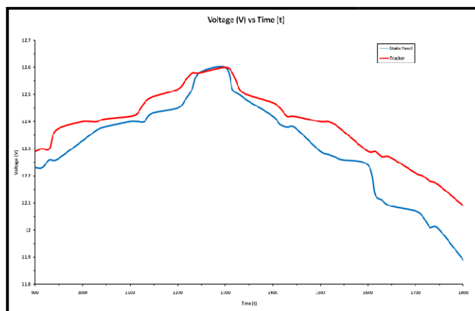
Figure 7. Output voltage comparison between static panel and tracker
