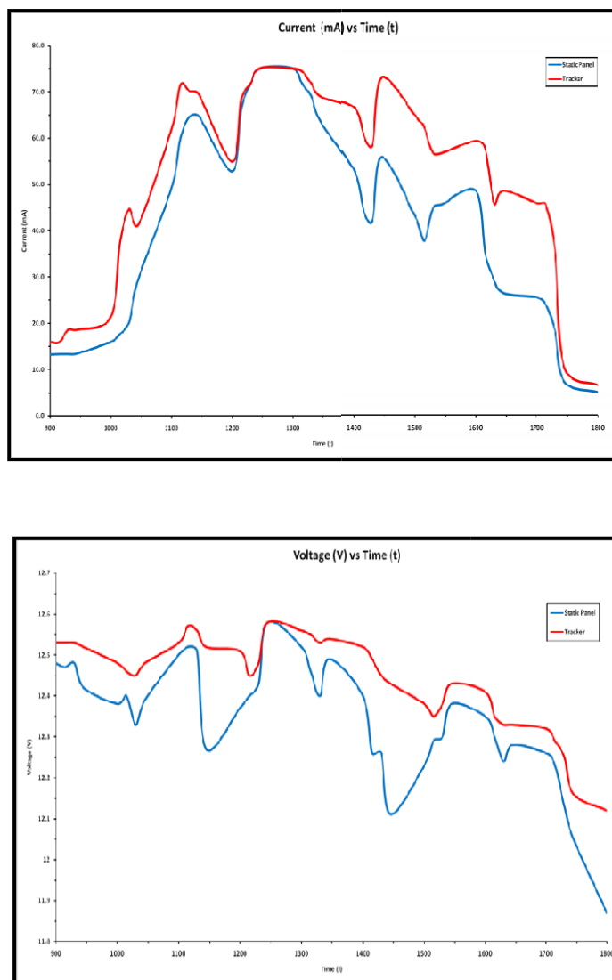
Figure 11. Output current comparison between static panel and tracker panel at most of the times.
