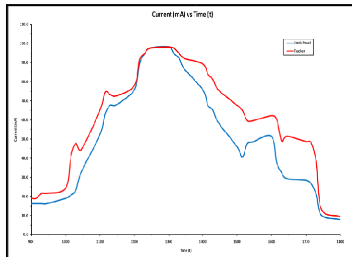
Figure 8. Output current comparison between static panel and tracker
