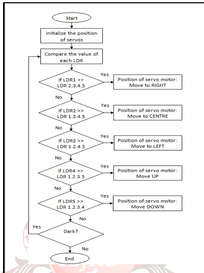
Figure 6. Flow chart of software
